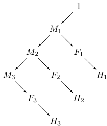
Figure 1: Graph for Echinacea aster data. Arrows go from parent nodes to child nodes. Nodes are labelled by their associated variables. The only root node is associated with the constant variable 1. M_j is the mortality status in year 2001 + j . F_j is the flowering status in year 2001 + j . H_j is the flower head count in year 2001 + j . The M_j and F_j are Bernoulli conditional on their parent variables being one, and zero otherwise. The H_j are zero-truncated Poisson conditional on their parent variables being one, and zero otherwise.
