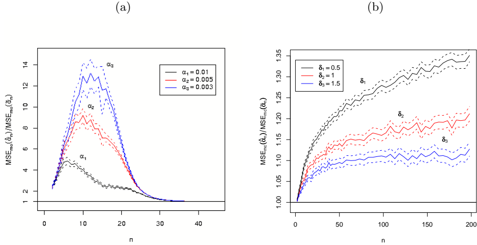
FIG 2. (a) Monte Carlo Mean Squared Error ratio computed from B = 10000 samples of size n , for different values of the true probability ( \alpha = .01, .005, .003 ). The distortion parameter is computed as q_n = [1/2 + e^{0.3(n-20)}] / [1 + e^{0.3(n-20)}] . (b) Monte Carlo Mean Squared Error ratio computed from B = 10000 samples of size n . We use sequences q_n = 1 - [10 \log(n + 10)]^{-1} and x_n = n^{\frac{1}{2+\delta}} ( \delta = 0.5, 1.0 and 1.5 ). The dashed lines represent 99% confidence bands.
