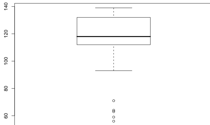
Boxplot
