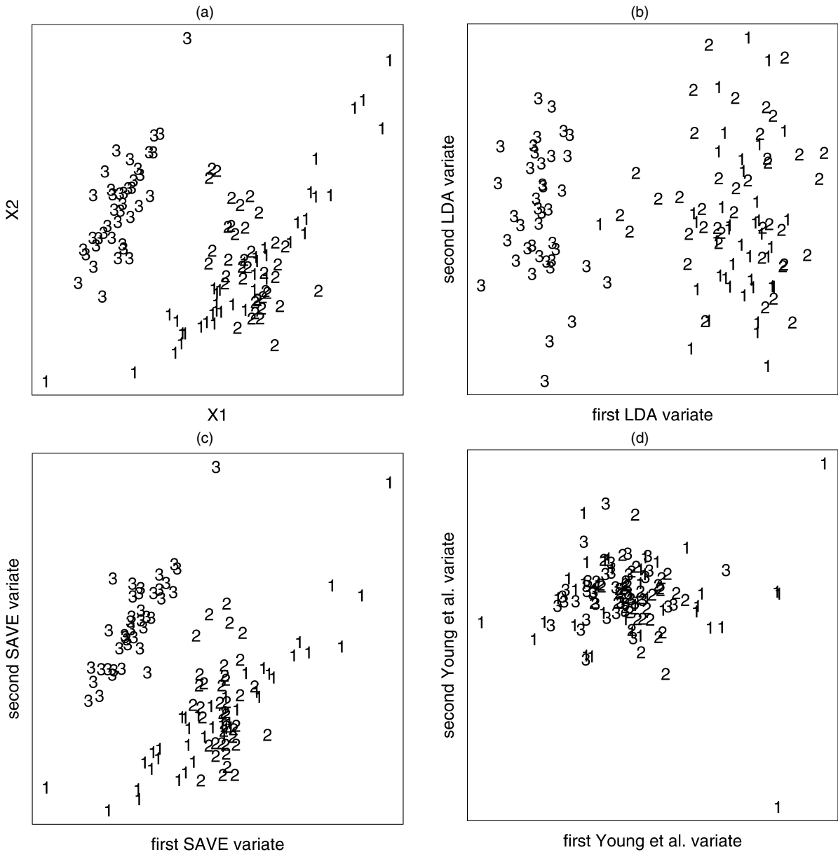
Figure 7. Scatterplots for the Constructed Robustness Example. (a) The first two feature variables representing the true dimension-reduction subspace; (b) the first two LDA canonical variates; (c) the first two SAVE variates; (d) the first two variates found using the method of Young et al.
