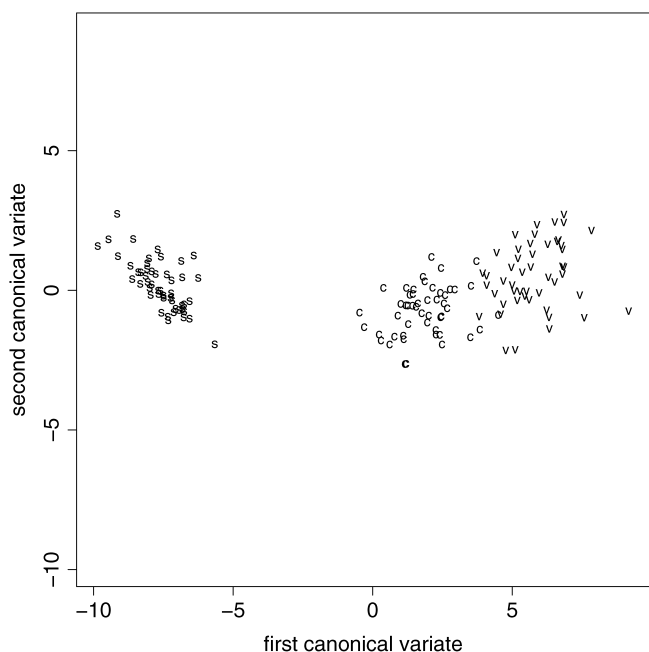
Figure 1. R LDA Graphical Display for the Iris Data. The scatterplot graphs the first sample canonical variate against the second, with the data points marked by class: s represents Iris setosa ; c , Iris versicolor ; v , Iris virginica .
