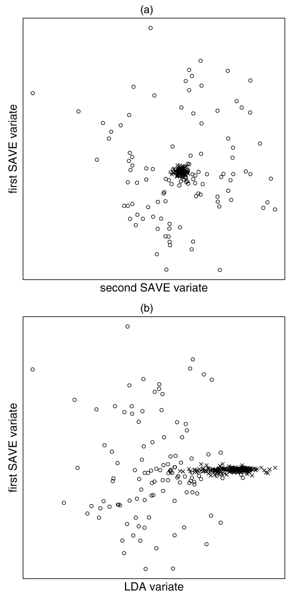
Figure 6. Scatterplots of SAVE Variates. (a) Scatterplot of the first two SAVE variates for the ionosphere data. The 225 good cases are indicated with crosses, which all fall near the center of the plot. (b) Scatterplot of the first SAVE variate and LDA variate.
