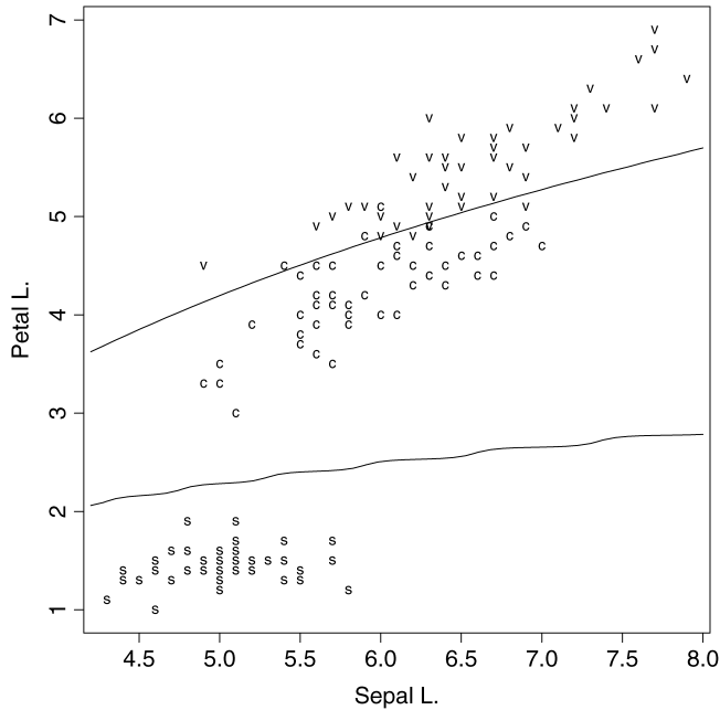
Figure 2. R QDA Graphical Display With Two Feature Variables for the Iris Data. The scatterplot graphs the first feature against the second, with the data points marked by class. The curved boundaries mark the quadratic classification regions.
