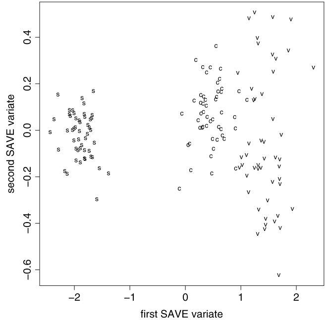
Figure 4. SAVE Summary Plot for the Iris Data. Here s represents Iris setosa ; c , Iris versicolor ; v , Iris virginica .
