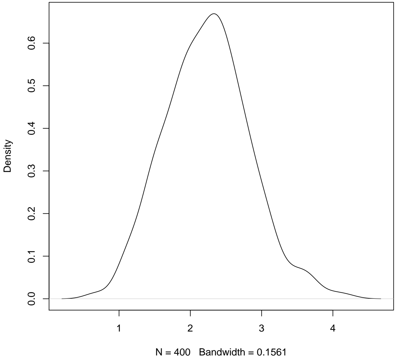
Series: \beta_{\text{victim}} spacing of chain 250
