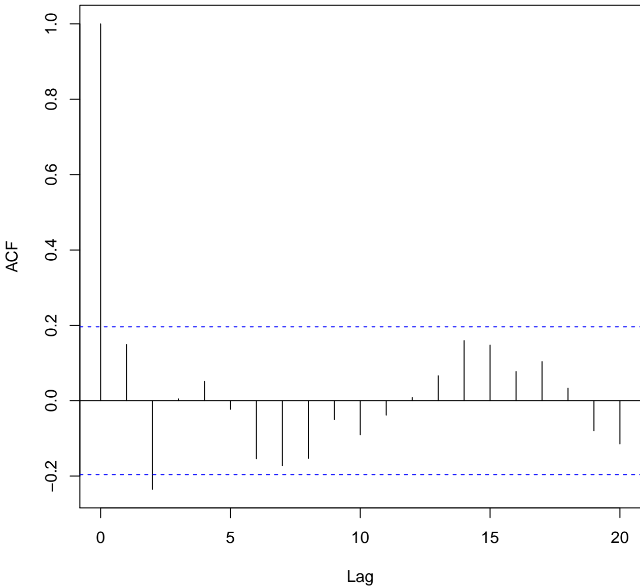
Series: \beta_{\text{defendant}} means of batches of length 100
