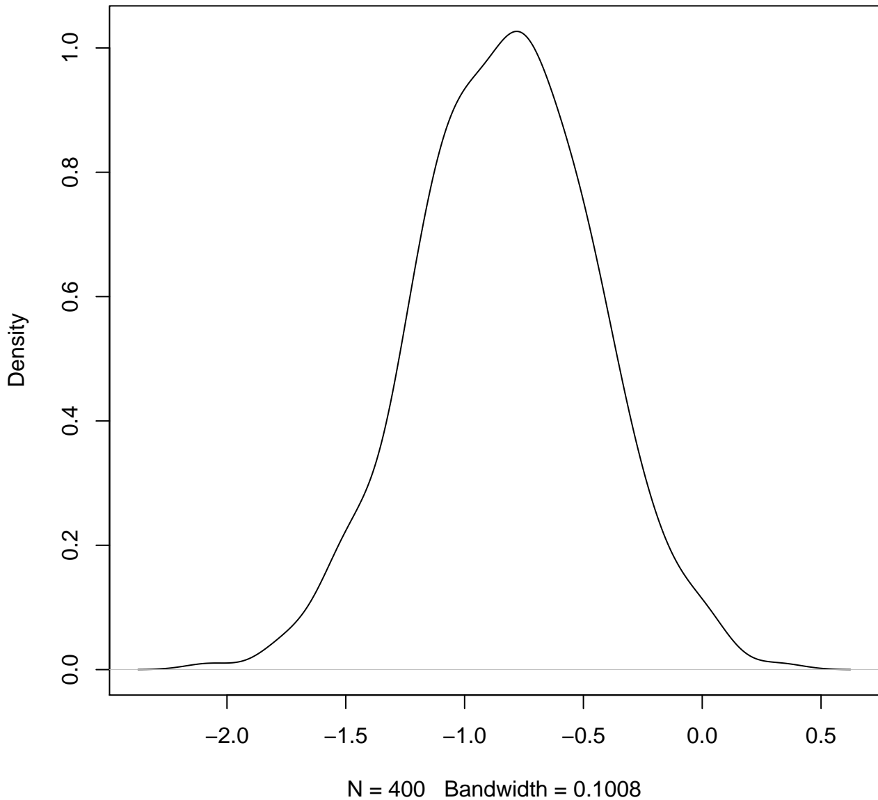
Series: \beta_{\text{defendant}} spacing of chain 250
