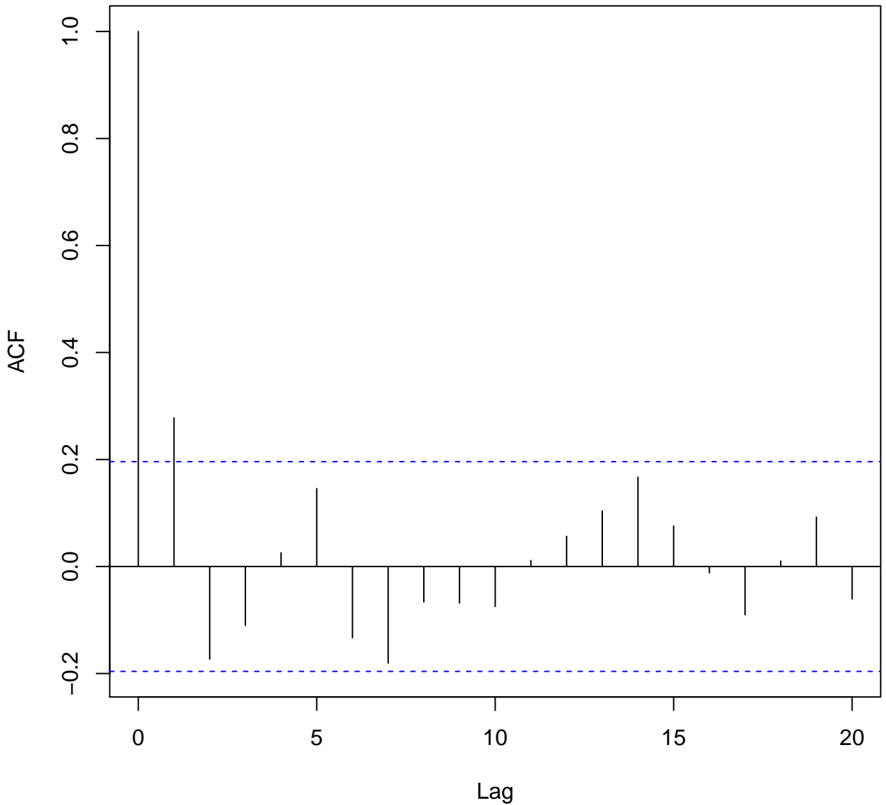
Series: \beta_{\text{victim}} means of batches of length 100
