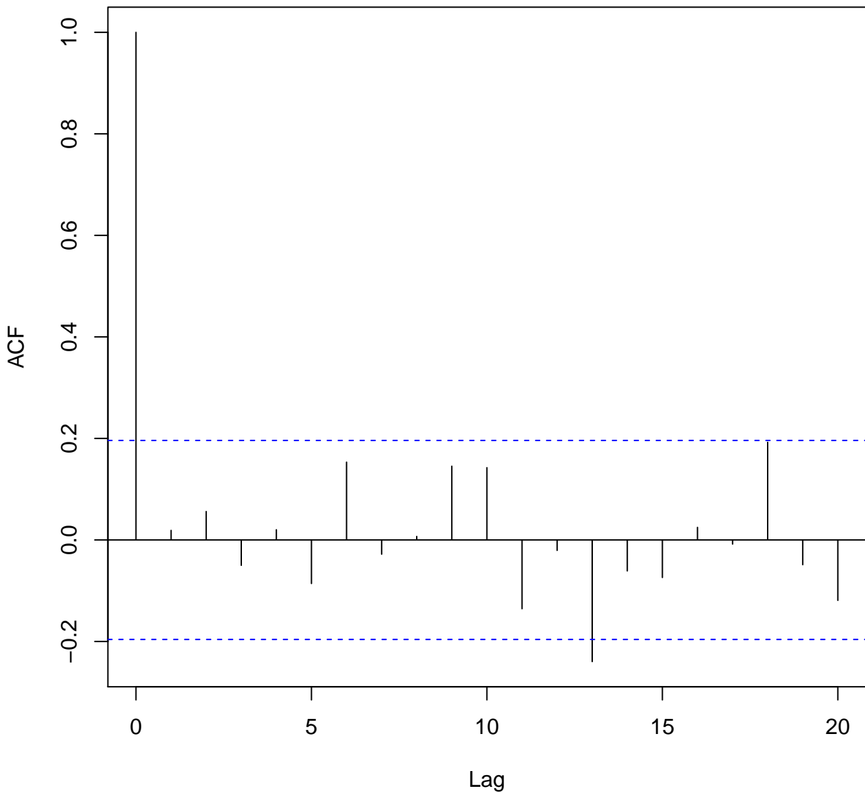
Series: \beta_{\text{defendant}} means of batches of length 250
