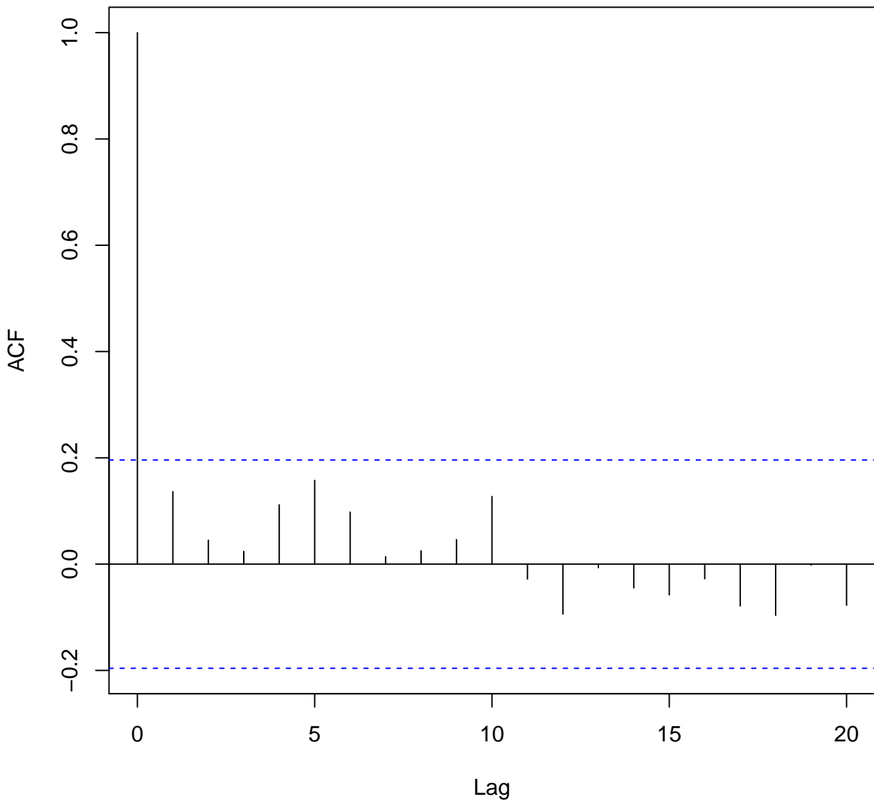
Series: \beta_{\text{victim}} means of batches of length 250
