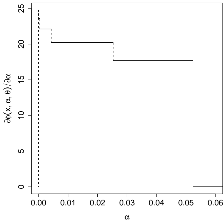
Figure 3: The density of the randomized P -value for the UMPU (two-tailed) test with binomial data x = 10 and n = 10 and null hypothesis \theta = 0.7 . The plotted step function has five steps. The intervals of constancy are the intervals in (1.5). The heights are the coefficients of \alpha in (1.5).
