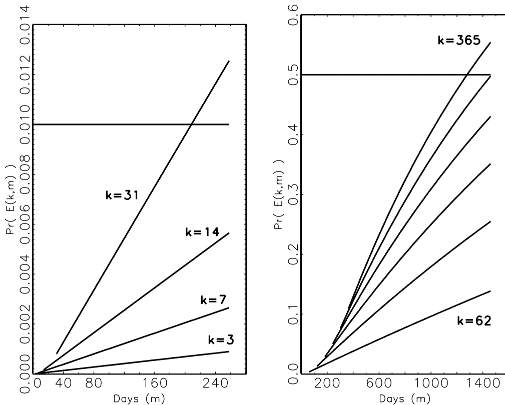
Figure 1. Probabilities p(k, m) , m \geq k . Left panel: k = 3, 7, 14, 31 ; m = k, \dots, 258 ; horizontal line at 0.01. Right panel: k corresponding to 2, 4, \dots , 12 months; m = k, \dots, 1460 (four years); horizontal line at 0.50. Continuous curves have been drawn for clarity even though the domain of p(k, \cdot) is discrete.
